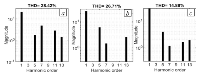
Fig. 5. The simulation harmonic spectrum of the inverter's output voltage: a – case 1; b – case 2; c – case 3
