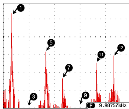
Fig. 12. The experimental harmonic spectrum of the 5-level output voltage in case 3
