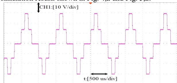
Fig. 7. The experimental output voltage of the 5-level inverter using SHE modulation in case 1
