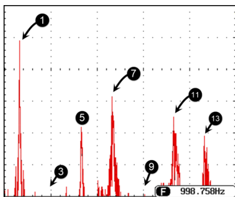
Fig. 8. The experimental harmonic spectrum of the 5-level output voltage in case 1
