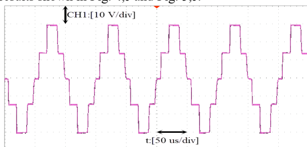
Fig. 11. The experimental output voltage of the 5-level inverter using SHE modulation in case 3
