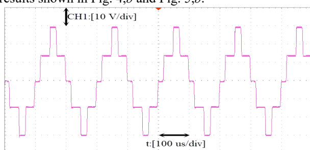
Fig. 9. The experimental output voltage of the 5-level inverter using SHE modulation in case 2
