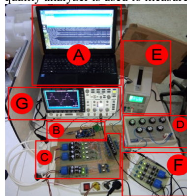
Fig. 6. Photo of the experimental setup: A – PC with Arduino IDE software B – Arduino Mega 2560 chip C – 5-level inverter D – resistive load E, F – power supplies G – oscilloscope
