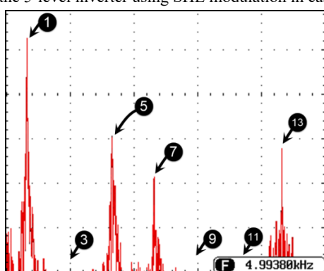
Fig. 10. The experimental harmonic spectrum of the 5-level output voltage in case 2
