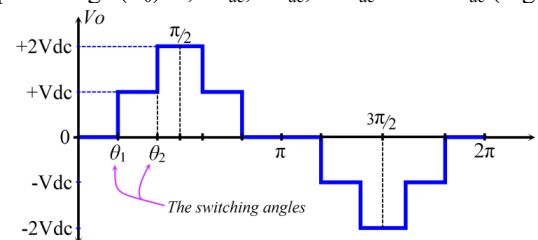
Fig. 2. The output voltage of the 5-level emerging inverter
