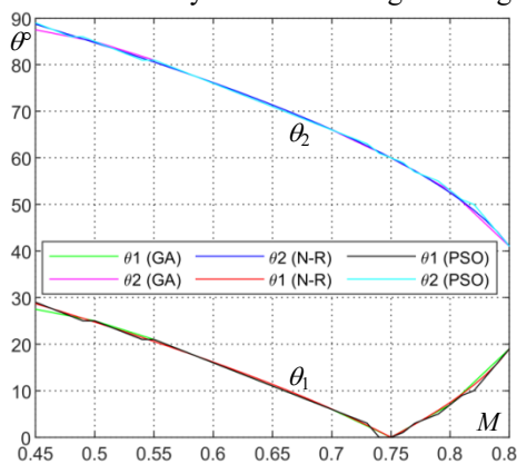
Fig. 3. The angles \theta_1 and \theta_2 versus M using the 3 algorithms
