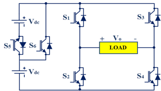
Fig. 1. Topology of the 5-level emerging inverter
