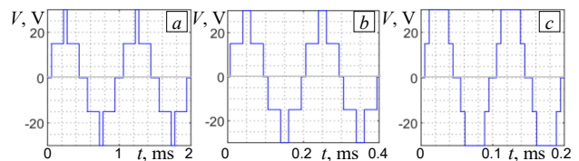
Fig. 4. The simulation output voltage of the 5-level inverter using SHE modulation: a – case 1; b – case 2; c – case 3
