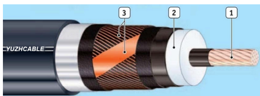
Fig. 1. Single-core XLPE-insulated power cable: 1 – aluminum or copper conductor, 2 – XLPE insulation, 3 – copper sheath
