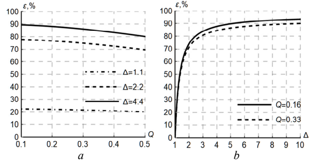
Fig. 2. Quality analysis of the regulatory formula for sheath current in the trefoil cable line
