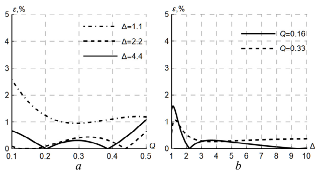
Fig. 4. Quality analysis of the novel approximation for sheath current in the flat cable line
