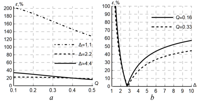
Fig. 3. Quality analysis of the regulatory formula for sheath current in the flat cable line
