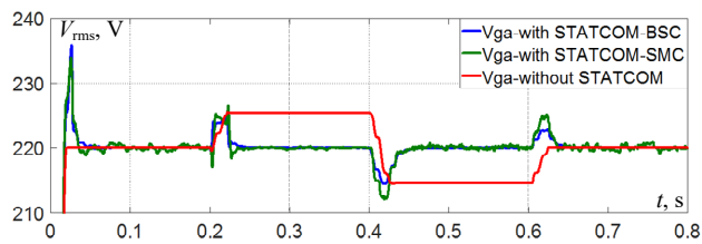
Fig. 6. RMS phase voltage at PCC without and with STATCOM
