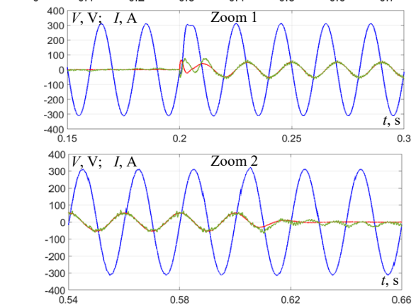
Fig. 10. Grid voltage V_{ga} and current I_{ca} waveform of STATCOM output
