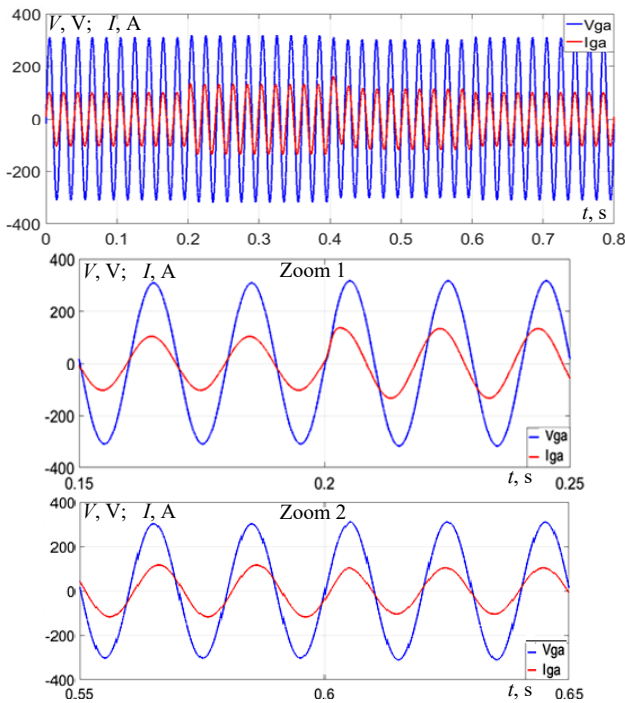
Fig. 12. Grid voltage V_{ga} and current I_{ga} without STATCOM
