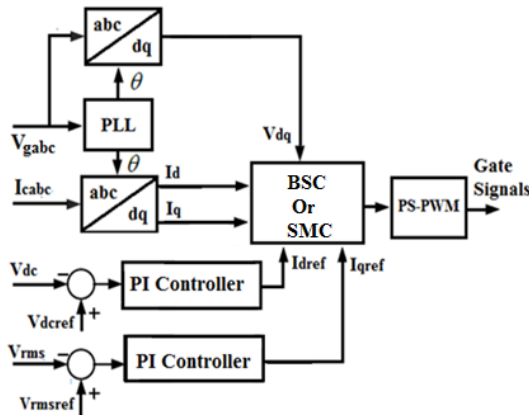
Fig. 3. STATCOM control block diagram
