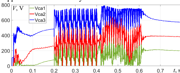
Fig. 18. Voltages of the flying capacitors in the FCMC
