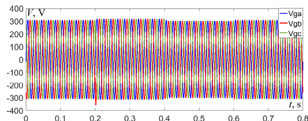
Fig. 7. 3-phase voltage (abc) at PCC without STATCOM
