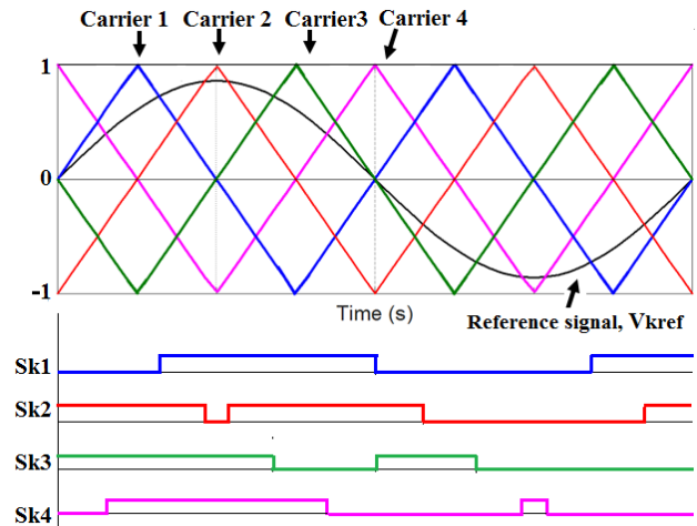
Fig. 4. PS-PWM technique for the 5-level FCMC
