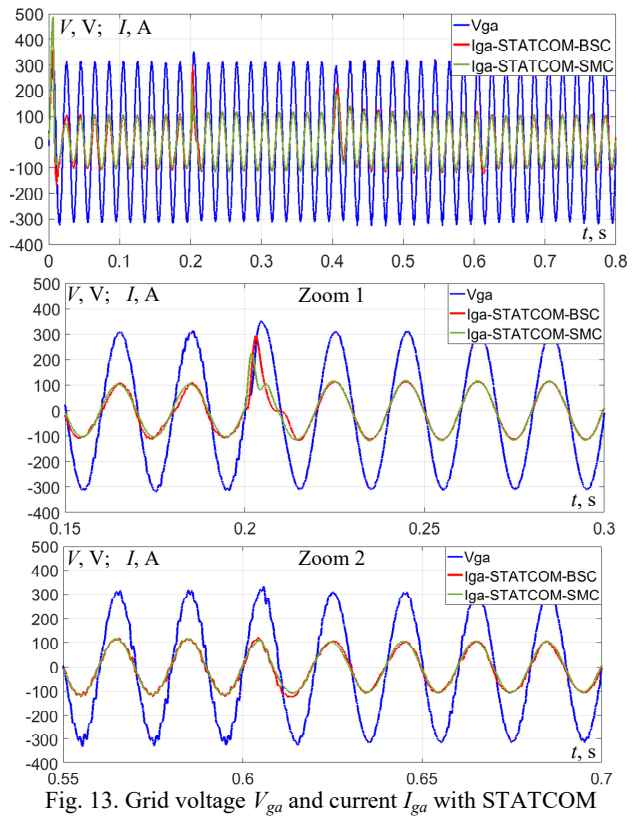
Fig. 13. Grid voltage V_{ga} and current I_{ga} with STATCOM
