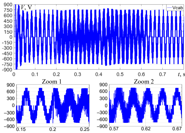
Fig. 16. Line-to-line output voltage V_{cab} of the STATCOM-BSC converter
