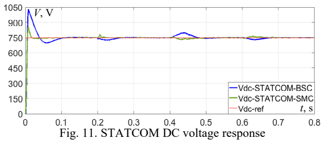
Fig. 11. STATCOM DC voltage response
