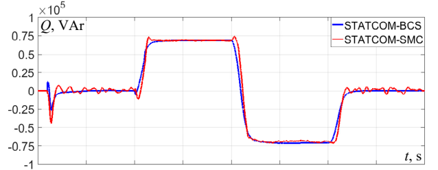
Fig. 9. Reactive power exchanged by the STATCOM
