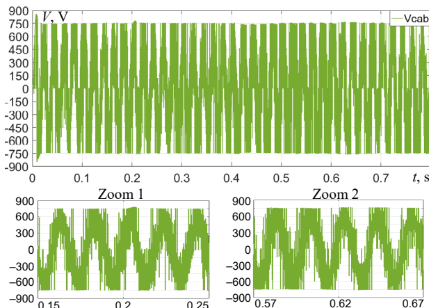
Fig. 17. Line-to-line output voltage V_{cab} of the STATCOM-SMC converter
