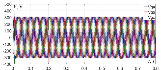
Fig. 8. 3-phase voltage (abc) at PCC with STATCOM
