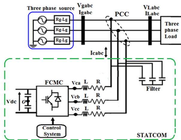
Fig. 1. Equivalent circuit of STATCOM
