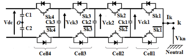
Fig. 2. Per-leg circuit configurations of the 5-level FCMC
