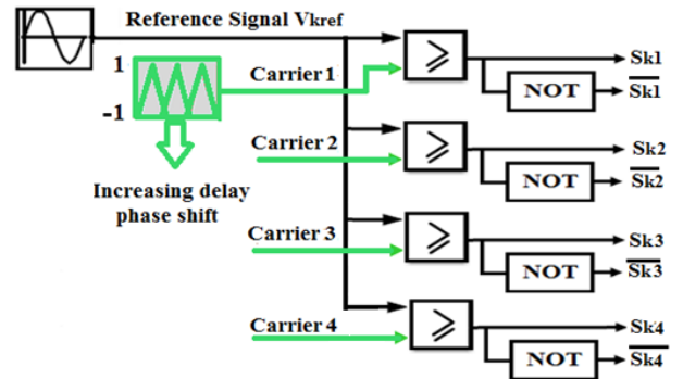
Fig. 5. Schematic diagram of the PS-PWM control
