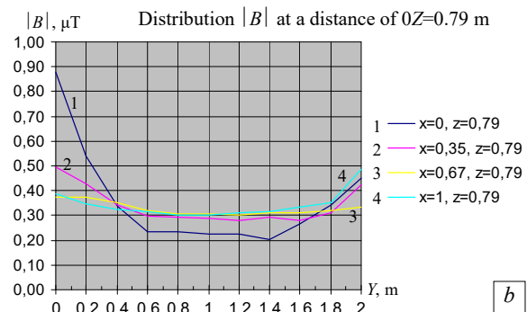
Fig. 11. Experimentally measured three dimensions magnetic field level distribution with combined shield with solid passive shield
