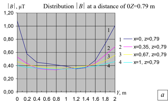
Fig. 10. Experimentally measured three dimensions magnetic field level distribution with combined shield with multi-circuit passive shield
