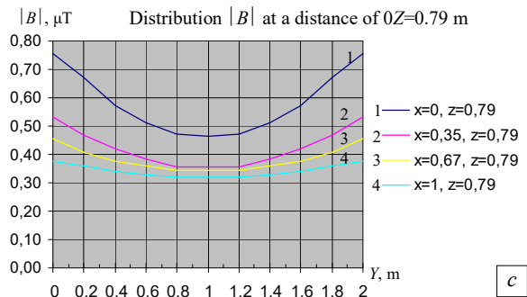
Fig. 10. Experimentally measured three dimensions magnetic field level distribution with combined shield with multi-circuit passive shield
