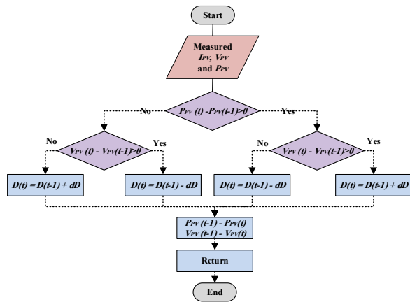
Fig. 5. The flowchart of P&O algorithm
