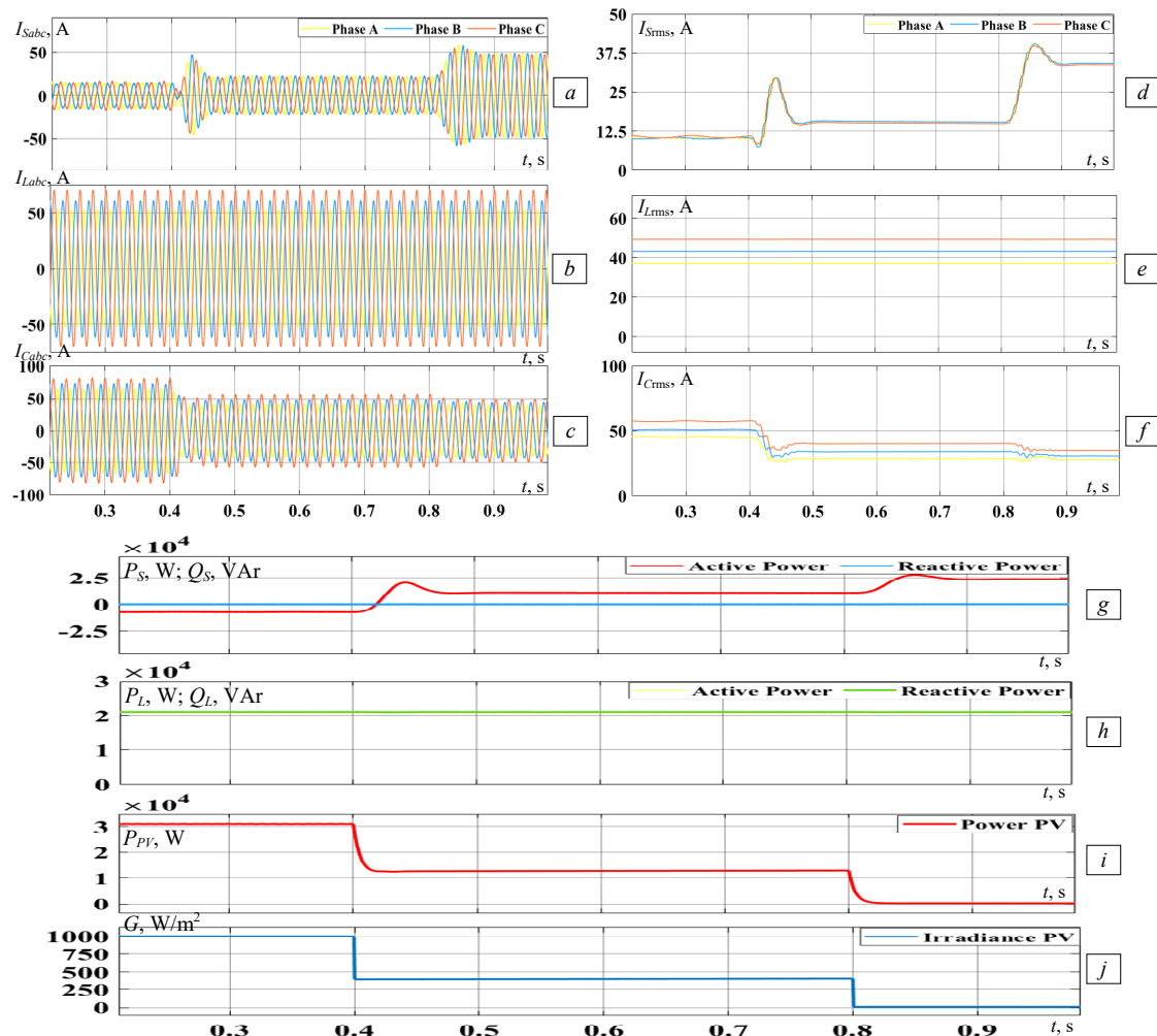
Fig. 7. All modes of the current quality issues in grid and load side: a – waveform grid current; b – waveform unbalance load current; c – current injected by shunt part of UPQC; d – RMS grid current; e – RMS of unbalance load current; f – RMS current injected by shunt part of UPQC; g – total active and reactive power of grid; h – total active and reactive power of load; i – total active PV power; j – solar radiation
