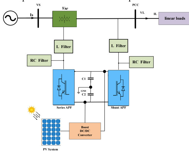
Fig. 1. Configuration of the UPQC-PV
