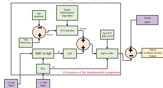
Fig. 3. The control circuit of shunt compensator in UPQC-based SRF technique
