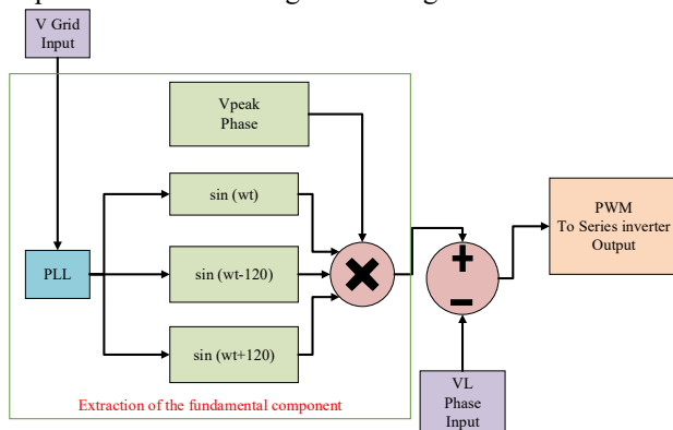
Fig. 2. The control circuit of series compensator in UPQC-based UVTG technique
