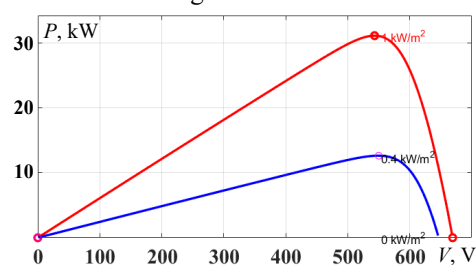
Fig. 4. P-V characteristics of PV panels
