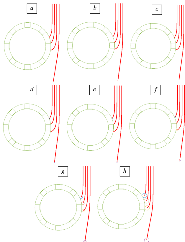
Fig. 7. Particle trajectories obtained for different particle sizes without considering the granular drag force:
