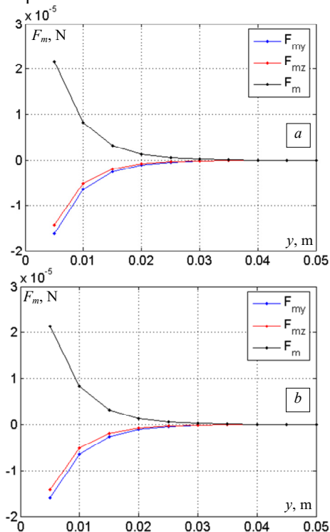
Fig. 6. Variation of the components of the magnetic force density as a function of the distance between the particle and the drum surface: a – Maxwell stress tensor method; b – field gradient method
