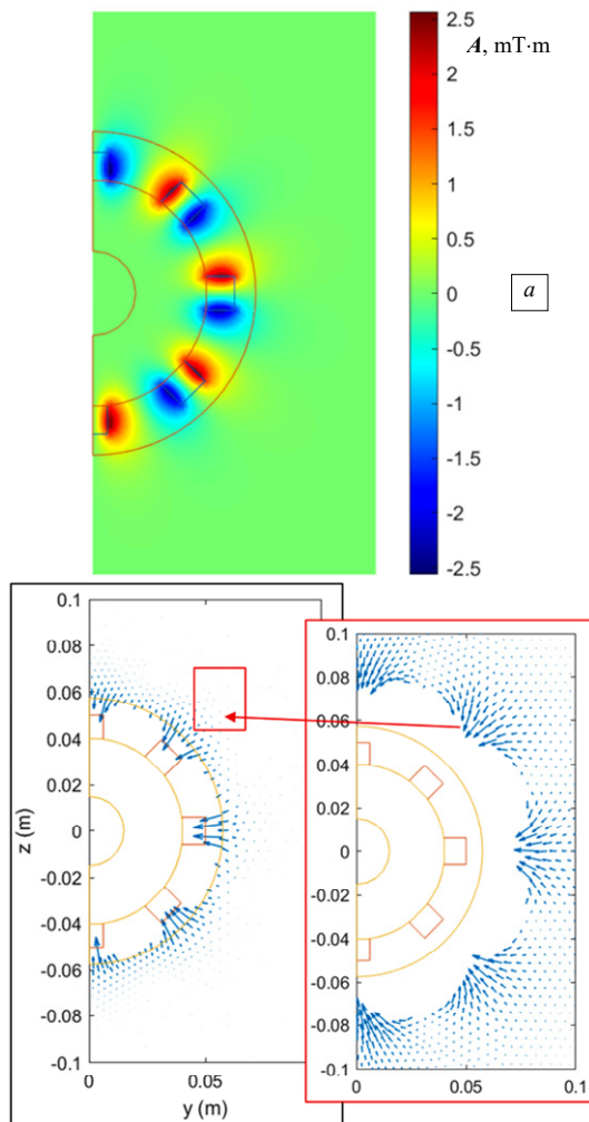
Fig. 2. Distributions of the magnetic field and force in the right side of the drum (plane (y, z) ): a – magnetic vector potential; b – magnetic force density
