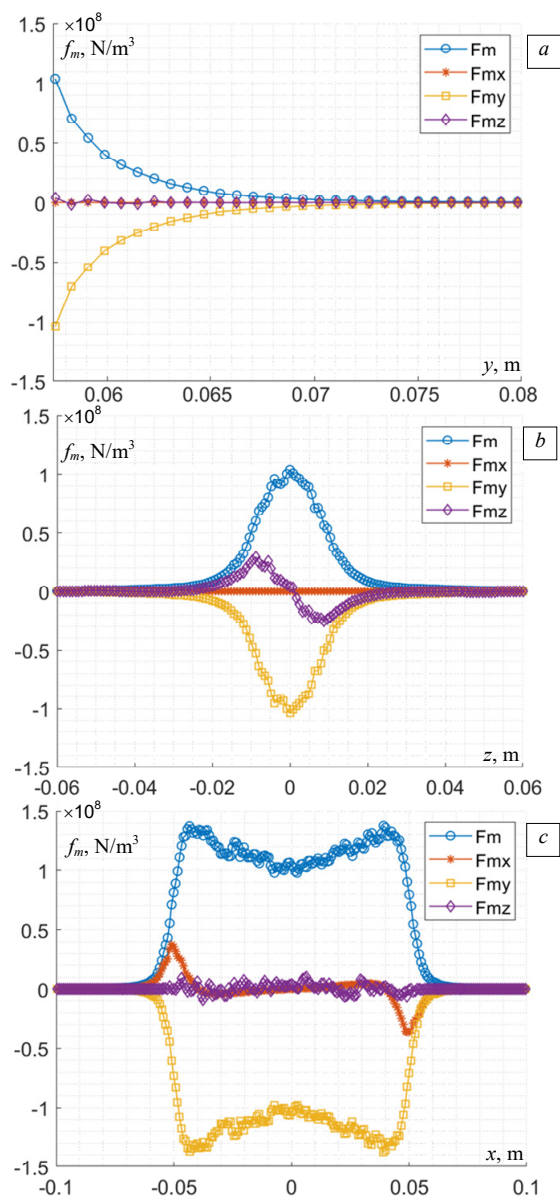
Fig. 4. Variations of the magnetic force density and its components ( F_{mx} , F_{my} , F_{mz} ) along the considered lines: a – line 2 (y direction); b – line 3 (z direction); c – line 1 (x direction)
