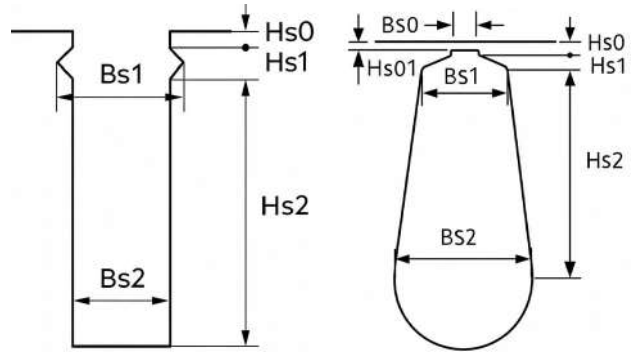
Fig. 1. Stator slot
