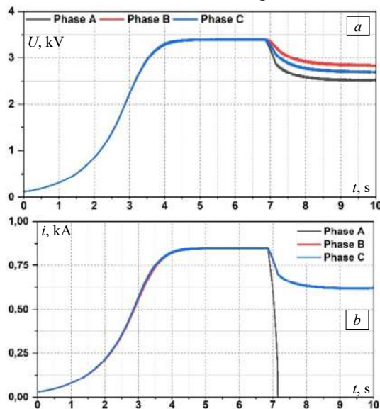
Fig. 11. RMS values of voltage (a) and current (b) under an open phase A condition
