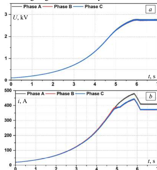
Fig. 12. RMS values of voltage (a) and current (b) under the condition of capacitor degradation
