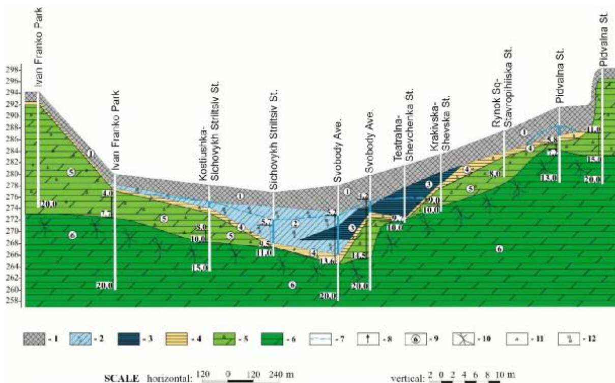
Fig. 4. Geological cross-section through the valley of the Poltava along the I-I line:
